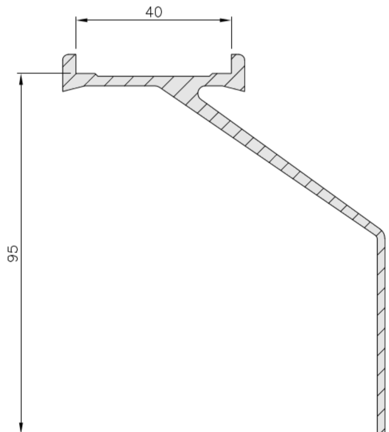
viprotech FLOODCOATER TYPE B Stock no. 38-90-025
